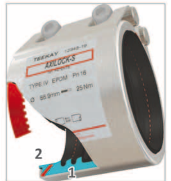
1 - multi-seal gasket 2 - encapsulated anchor ring
